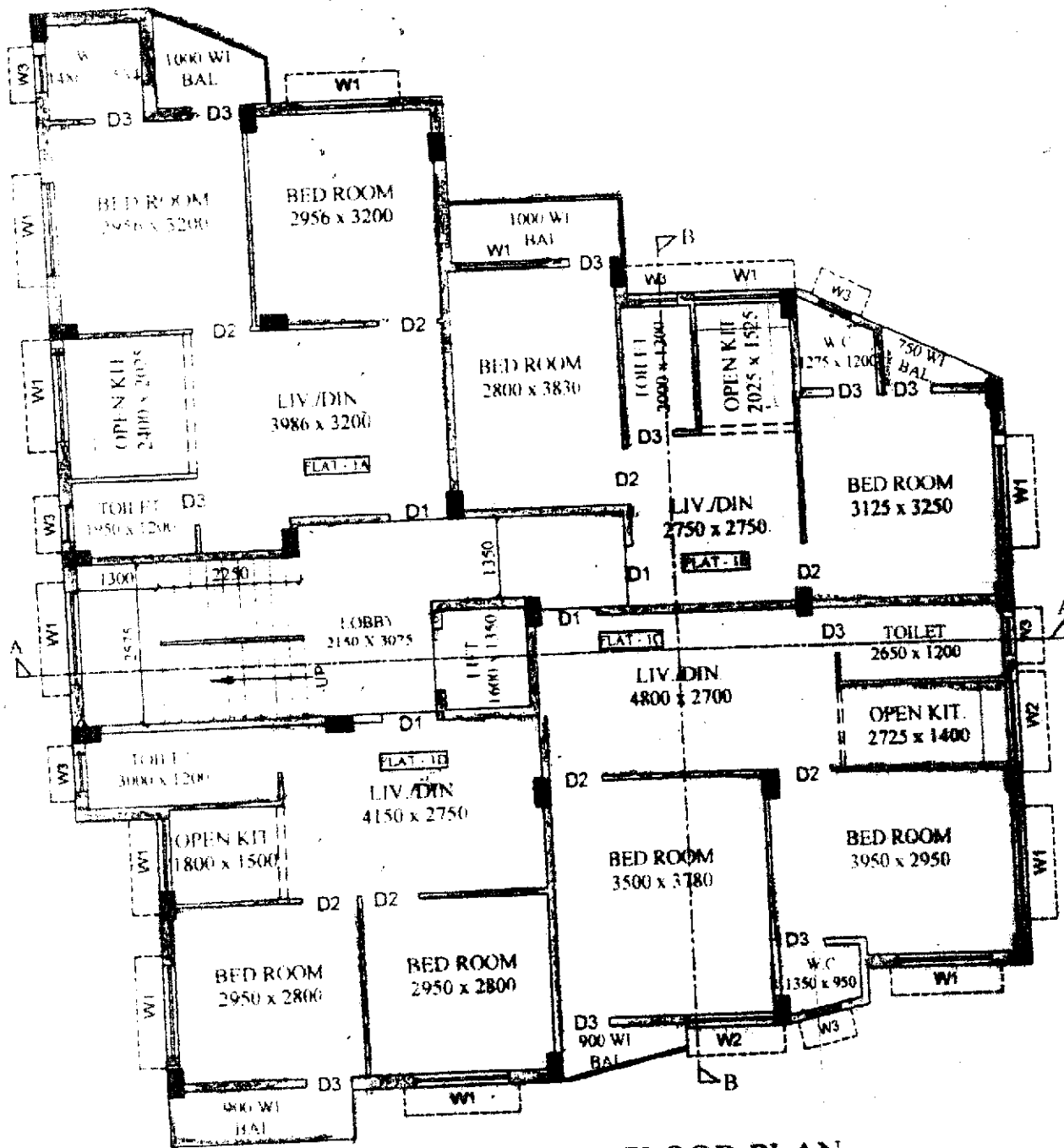
TYP. (1ST-4TH) FLOOR PLAN SCALE: 1:100
